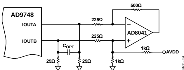
Figure 27. Single-Supply DC Differential Coupled Circuit
