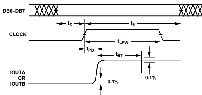
Figure 2. Timing Diagram
