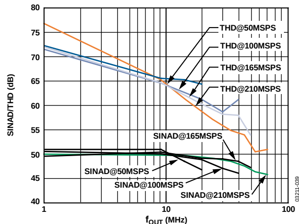
Figure 8. SINAD/THD vs. f_{OUT} (Single-Ended Output)
