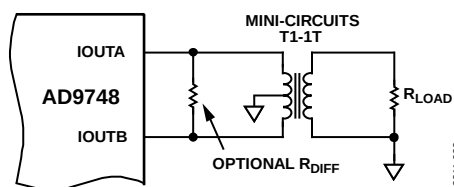
Figure 25. Differential Output Using a Transformer
