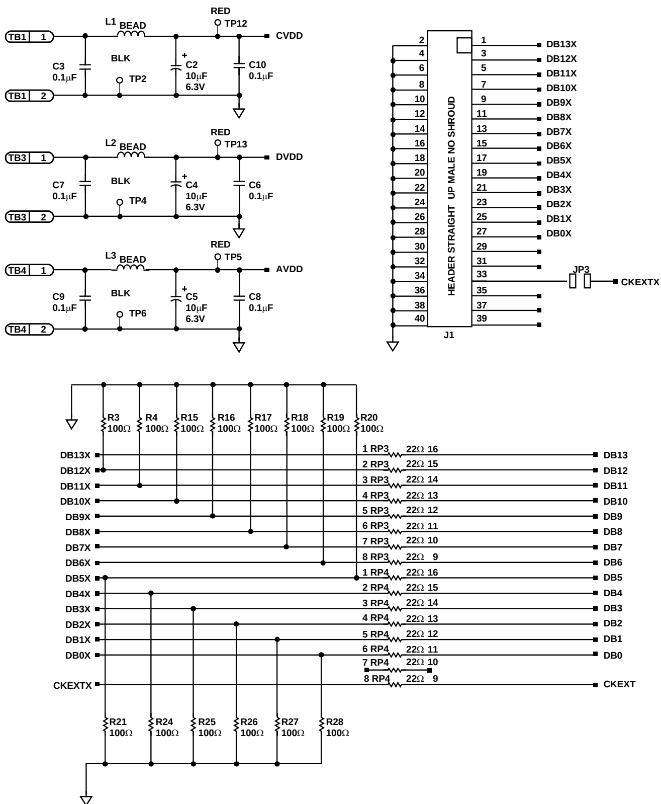
Figure 32. Evaluation Board Schematic—Power Supply and Digital Inputs
