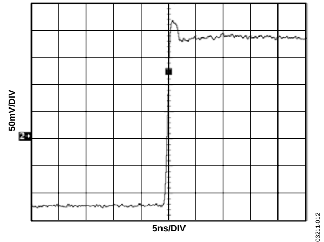
Figure 13. Step Response (Single-Ended Output)
