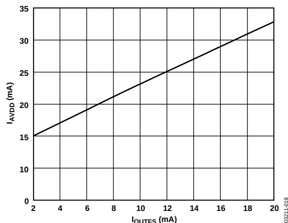
Figure 22. I_{AVDD} vs. I_{OUTFS}
