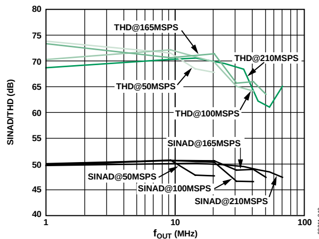
Figure 9. SINAD/THD vs. f_{OUT} (Differential Output)
