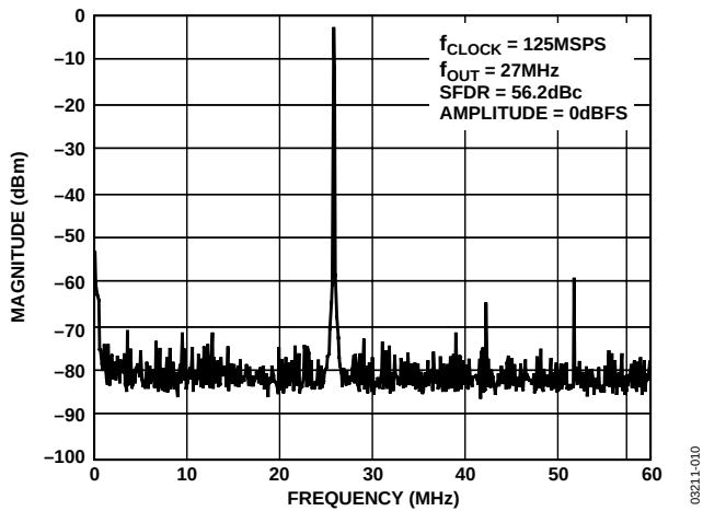
Figure 11. Single-Tone Spectral Plot @ 125 MSPS (Single-Ended Output)
