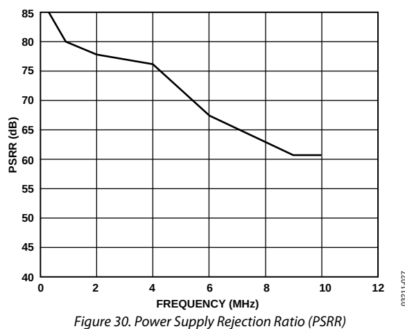
Figure 30. Power Supply Rejection Ratio (PSRR)
