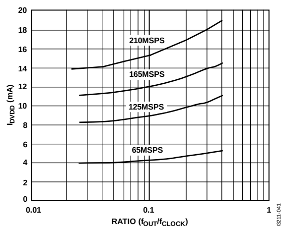
Figure 23. I_{DVDD} vs. Ratio @ DVDD = 3.3 V
