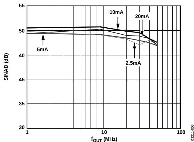
Figure 6. SINAD vs. f_{OUT} @ 165 MSPS (Single-Ended Output)
