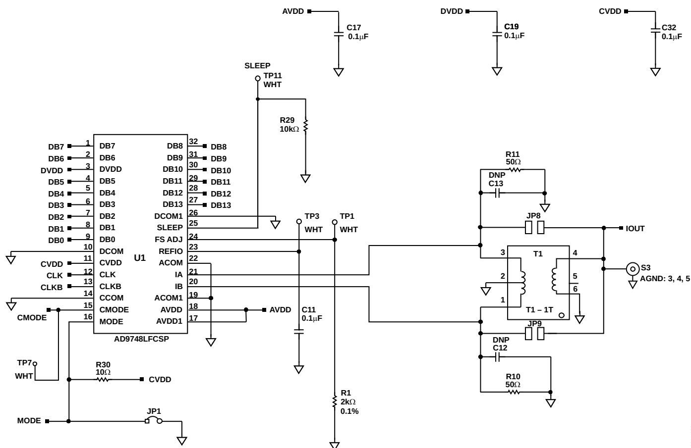
Figure 33. Evaluation Board Schematic—Output Signal Conditioning
