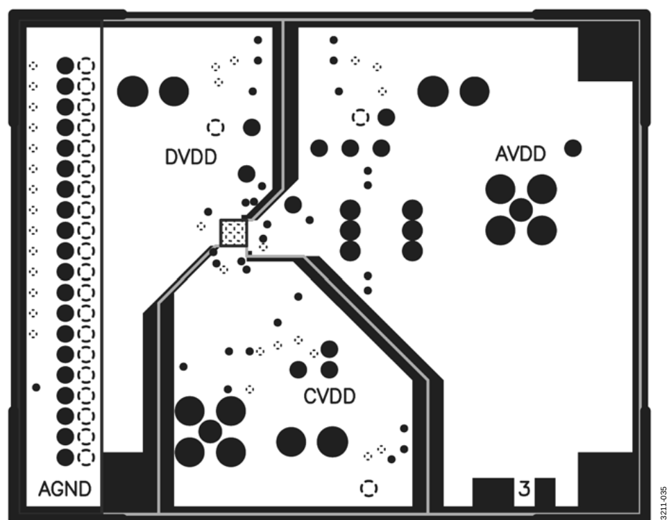
Figure 38. Evaluation Board Layout—Power Plane
