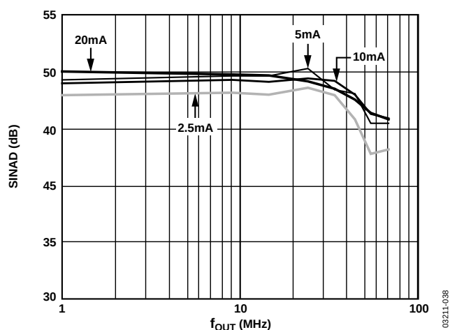
Figure 7. SINAD vs. f_{OUT} @ 210 MSPS (Single-Ended Output)
