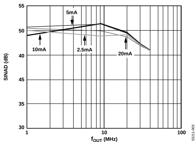
Figure 5. SINAD vs. f_{OUT} @ 100 MSPS (Single-Ended Output)
