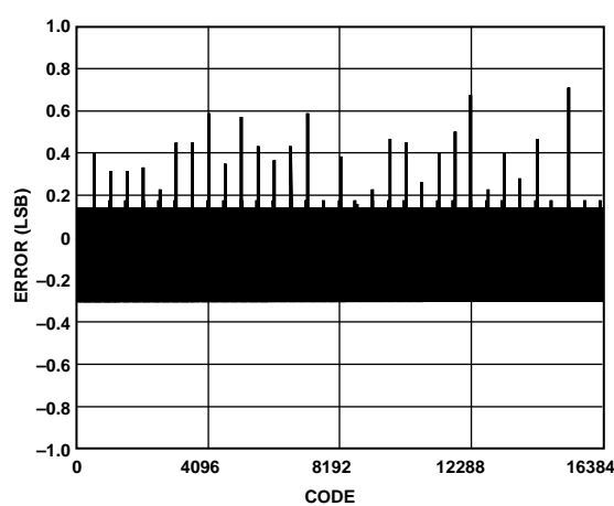
Figure 16. Typical DNL
