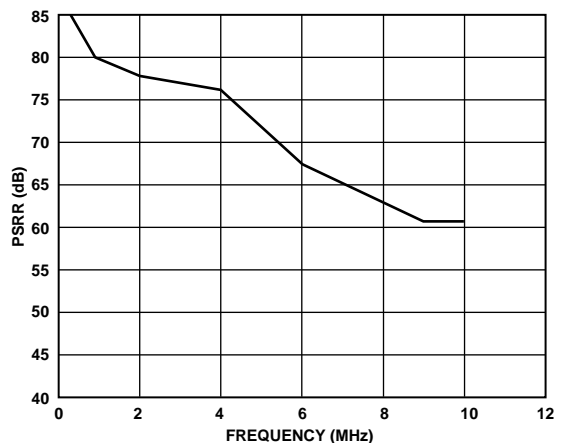
Figure 36. Power Supply Rejection Ratio (PSRR)
