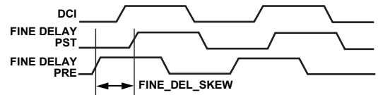
Figure 43. Pre- and Post-Delay Sampling Diagram
