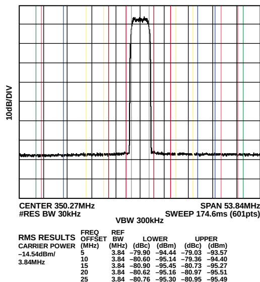
Figure 103. Single-Carrier WCDMA at 350 MHz, f_{DAC} = 2457.6 MSPS
