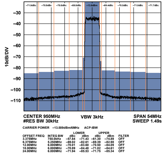
Figure 47. High Band Narrow-Band ACLR
