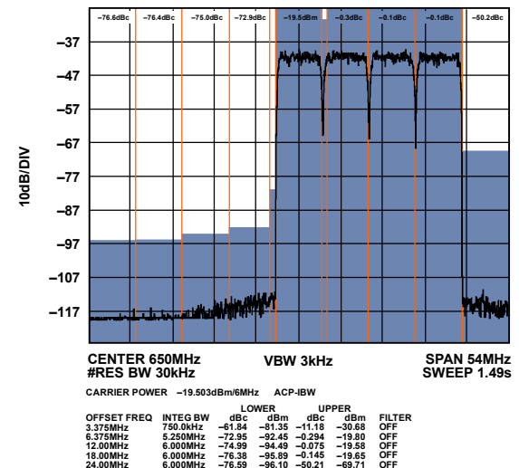
Figure 126. Mid Band Narrow-Band ACLR (Worse Side)
