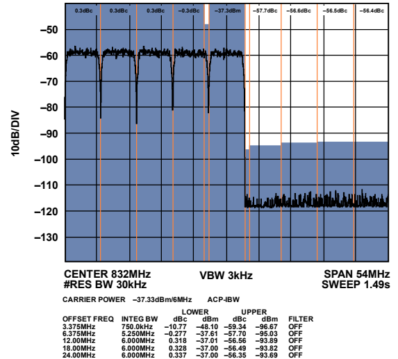
Figure 151. 128-Carrier Narrow-Band ACLR
