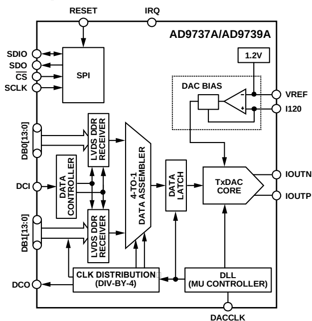
Figure 157. Functional Block Diagram of the AD9737A/AD9739A
