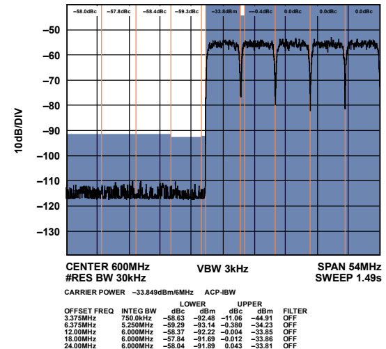
Figure 76. 64-Carrier High Band Narrow-Band ACLR
