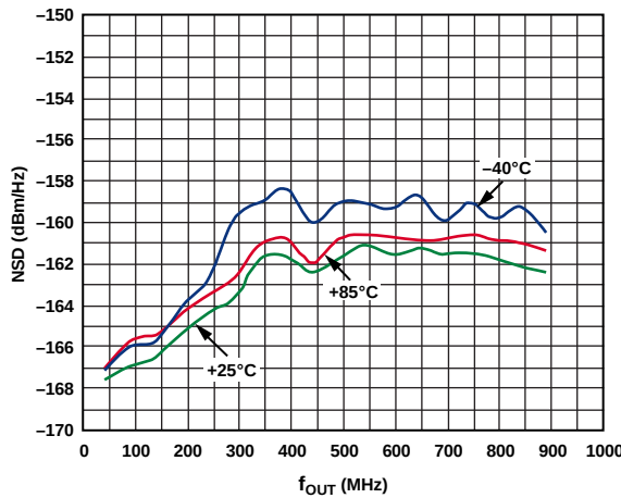
Figure 102. Single-Tone NSD vs. f_{OUT} over Temperature
