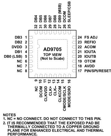
Figure 5. AD9705 Pin Configuration
