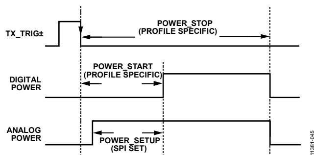
Figure 44. Power Sequencing
