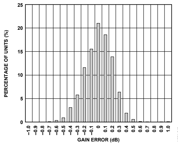
Figure 12. Gain Error Histogram, V_{\text{GAIN}} = 1.28 V
