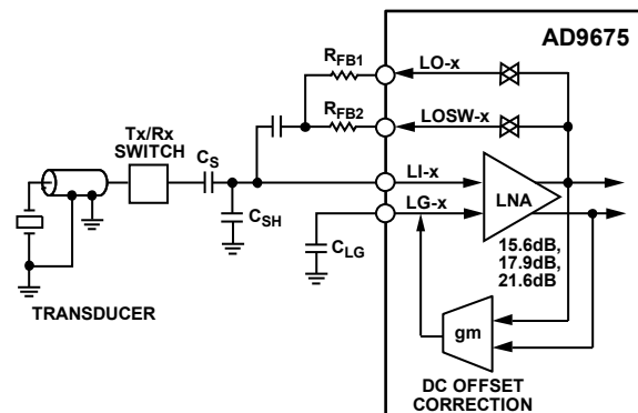
Figure 37. Simplified LNA Input Configuration
