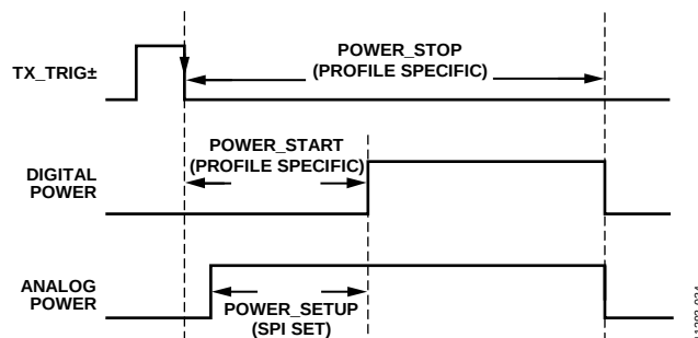
Figure 44. Power Sequencing
