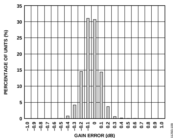
Figure 11. Gain Error Histogram, V_{\text{GAIN}} = 0 V
