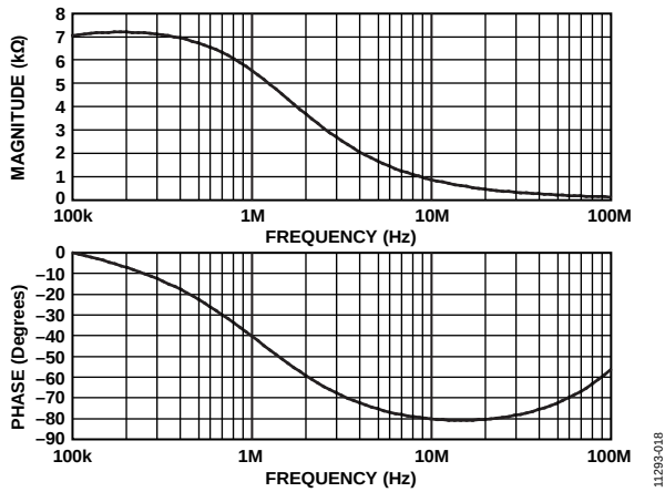
Figure 27. LNA Input Impedance Magnitude and Phase, Untermated
