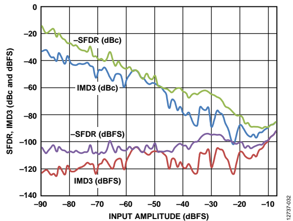
Figure 29. Two-Tone SFDR, IMD3 vs. Input Amplitude ( A_{IN} ) with f_{IN1} = 100.1 MHz and f_{IN2} = 102.1 MHz, f_{SAMPLE} = 125 MSPS, V_{REF} = 1.4 V
