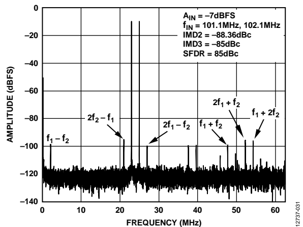
Figure 28. Two-Tone 32k FFT with f_{IN1} = 100.1 MHz and f_{IN2} = 102.1 MHz, f_{SAMPLE} = 125 MSPS, V_{REF} = 1.4 V
