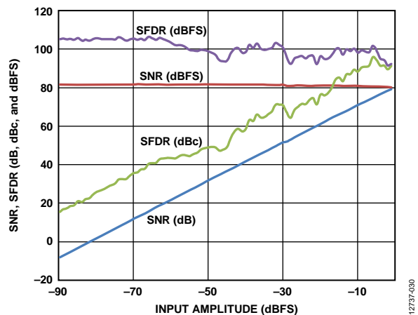
Figure 27. SNR, SFDR vs. Input Amplitude; f_{IN} = 9.7 MHz, f_{SAMPLE} = 125 MSPS, V_{REF} = 1.4 V
