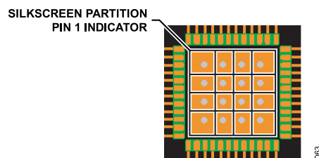
Figure 71. Typical PCB Layout
