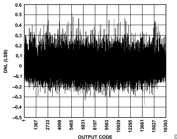
Figure 40. DNL; f_{IN} = 9.7 MHz, f_{SAMPLE} = 125 MSPS
