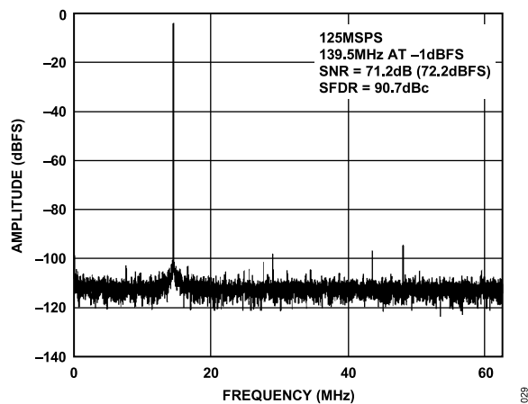
Figure 31. Single-Tone 16k FFT with f_{IN} = 139.5 MHz, f_{SAMPLE} = 125 MSPS
