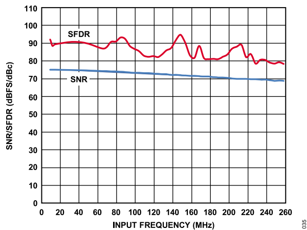
Figure 37. SNR/SFDR vs. f_{IN} ; f_{SAMPLE} = 125 MSPS
