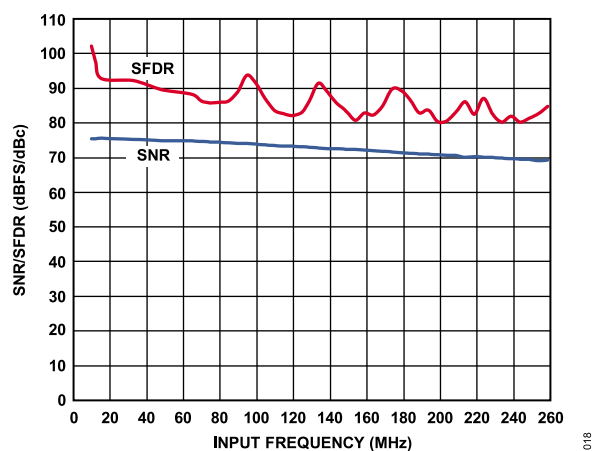
Figure 20. SNR/SFDR vs. f_{IN} ; f_{SAMPLE} = 80 MSPS
