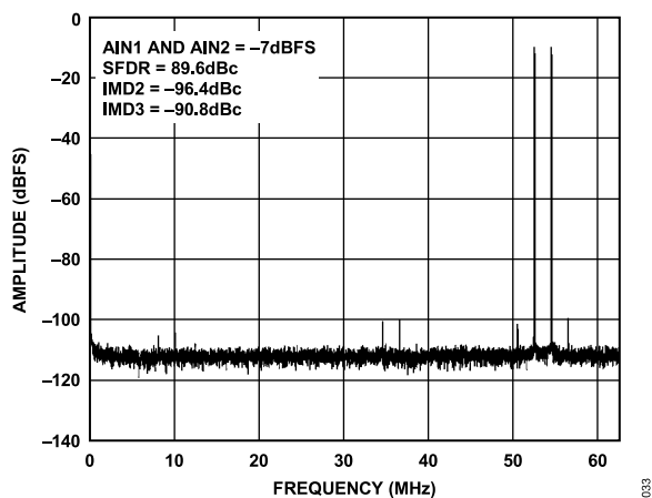
Figure 35. Two-Tone 16k FFT with f_{IN1} = 70.5 MHz and f_{IN2} = 72.5 MHz, f_{SAMPLE} = 125 MSPS
