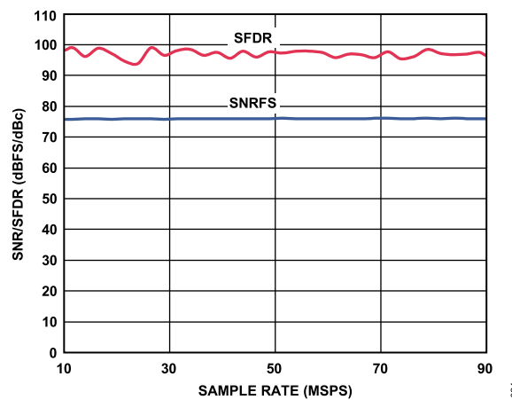
Figure 26. SNR/SFDR vs. Sample Rate; f_{IN} = 9.7 MHz, f_{SAMPLE} = 80 MSPS
