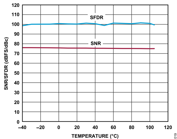
Figure 21. SNR/SFDR vs. Temperature; f_{IN} = 9.7 MHz, f_{SAMPLE} = 80 MSPS
