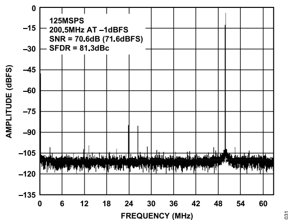
Figure 33. Single-Tone 16k FFT with f_{IN} = 200.5 MHz, f_{SAMPLE} = 125 MSPS, Clock Divide = Divide-by-8
