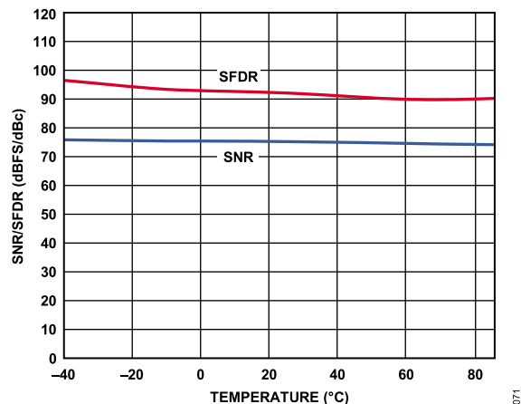
Figure 38. SNR/SFDR vs. Temperature; f_{IN} = 9.7 MHz, f_{SAMPLE} = 125 MSPS
