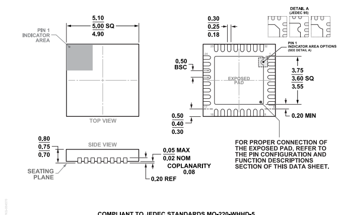
Figure 72. 32-Lead Lead Frame Chip Scale Package [LFCSP] 5 mm x 5 mm Body and 0.75 mm Package Height (CP-32-12) Dimensions shown in millimeters
