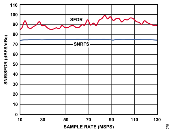
Figure 44. SNR/SFDR vs. Sample Rate; f_{IN} = 70 MHz, f_{SAMPLE} = 125 MSPS
