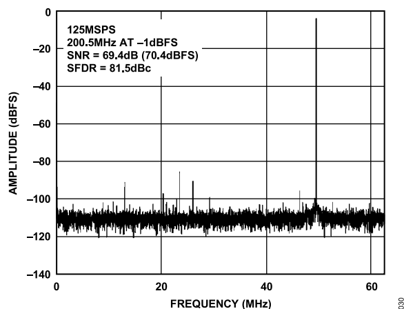
Figure 32. Single-Tone 16k FFT with f_{IN} = 200.5 MHz, f_{SAMPLE} = 125 MSPS
