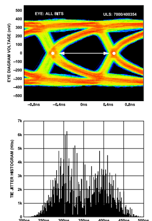
Figure 68. Data Eye for LVDS Outputs in ANSI-644 Mode with Trace Lengths of Less Than 24 Inches on Standard FR-4 Material, External 100 \Omega Far-End Termination Only
