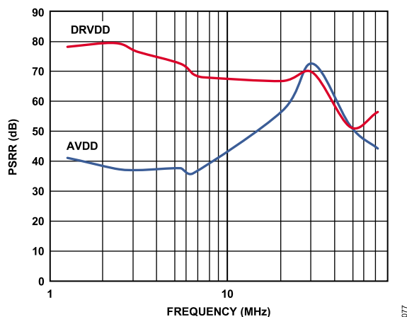
Figure 42. PSRR vs. Frequency; f_{CLK} = 125 MHz, f_{SAMPLE} = 125 MSPS
