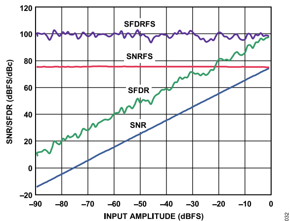
Figure 34. SNR/SFDR vs. Analog Input Level; f_{IN} = 9.7 MHz, f_{SAMPLE} = 125 MSPS
