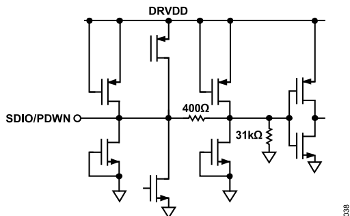
Figure 47. Equivalent SDIO/PDWN Input Circuit
