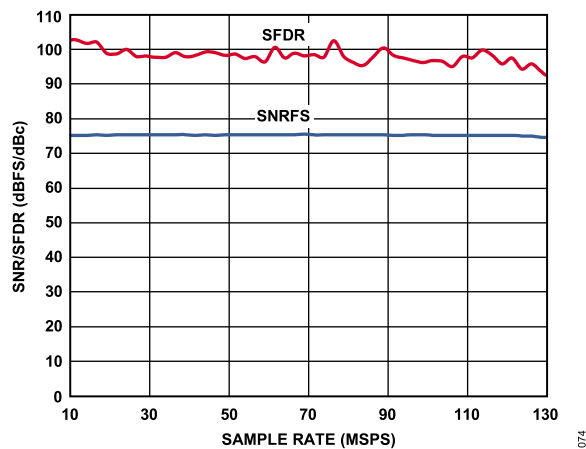
Figure 43. SNR/SFDR vs. Sample Rate; f_{IN} = 9.7 MHz, f_{SAMPLE} = 125 MSPS
