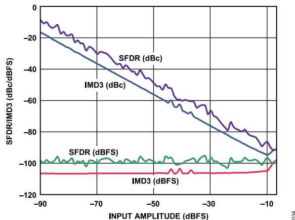
Figure 36. Two-Tone SFDR/IMD3 vs. Input Amplitude (AIN) with f_{IN1} = 70.5 MHz and f_{IN2} = 72.5 MHz, f_{SAMPLE} = 125 MSPS
