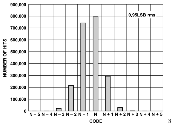
Figure 24. Input Referred Noise Histogram; f_{SAMPLE} = 80 MSPS
