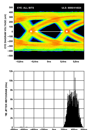
Figure 69. Data Eye for LVDS Outputs in ANSI-644 Mode with Trace Lengths Greater Than 24 Inches on Standard FR-4 Material, External 100 \Omega Far-End Termination Only
