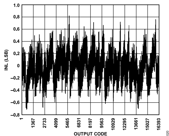
Figure 22. INL; f_{IN} = 9.7 MHz, f_{SAMPLE} = 80 MSPS
