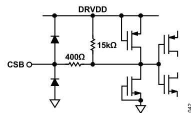
Figure 51. Equivalent CSB Input Circuit
