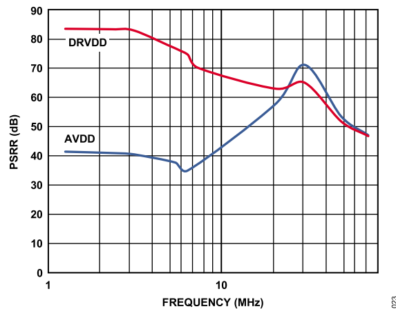
Figure 25. PSRR vs. Frequency; f_{CLK} = 125 MHz, f_{SAMPLE} = 80 MSPS
