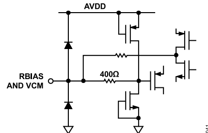
Figure 50. Equivalent RBIAS and VCM Circuit
