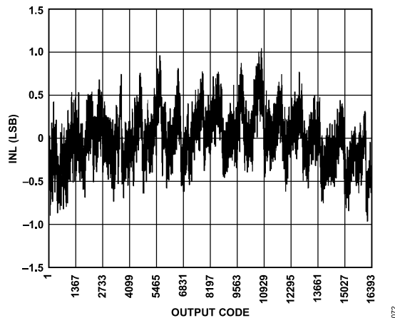
Figure 39. INL; f_{IN} = 9.7 MHz, f_{SAMPLE} = 125 MSPS
