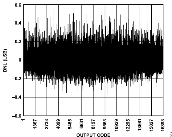
Figure 23. DNL; f_{IN} = 9.7 MHz, f_{SAMPLE} = 80 MSPS
