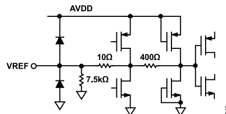
Figure 52. Equivalent VREF Circuit
