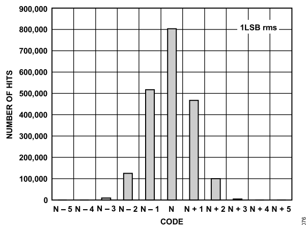
Figure 41. Input Referred Noise Histogram; f_{SAMPLE} = 125 MSPS
