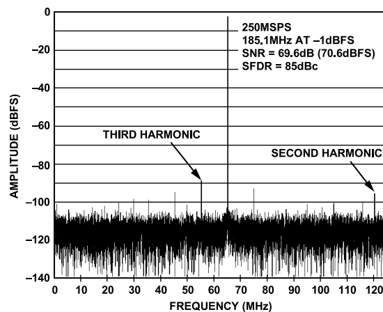
Figure 29. AD9643-250 Single-Tone FFT with f_{IN} = 185.1 MHz
