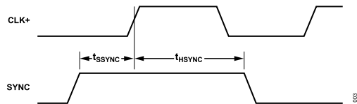
Figure 3. SYNC Timing Inputs
