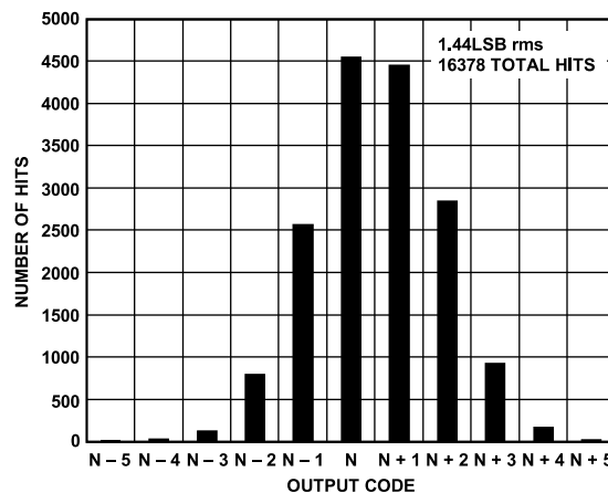
Figure 27. AD9643-210 Grounded Input Histogram
