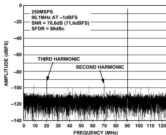
Figure 28. AD9643-250 Single-Tone FFT with f_{IN} = 90.1 MHz
