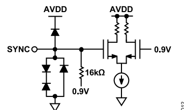
Figure 45. Equivalent SYNC Input Circuit
