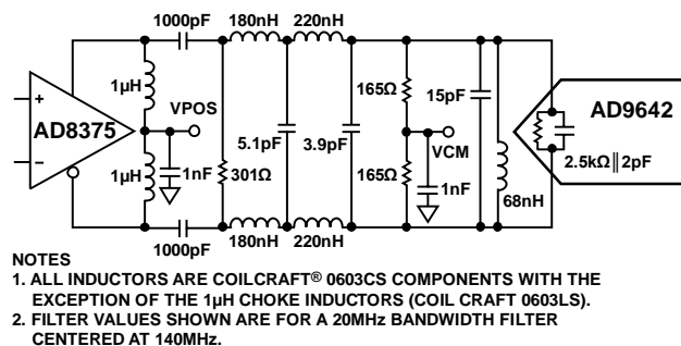
Figure 49. Differential Input Configuration Using the AD8375
