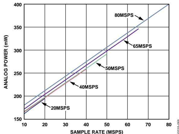
Figure 56. Analog Core Power vs. f_{\text{SAMPLE}} for f_{\text{IN}} = 9.7 MHz
