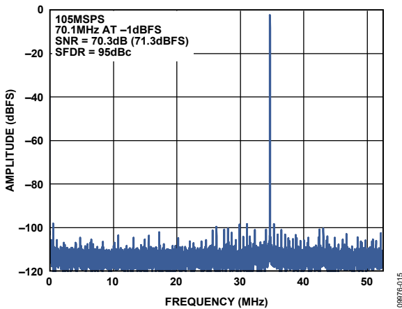
Figure 25. Single-Tone FFT with f_{IN} = 70.1 MHz
