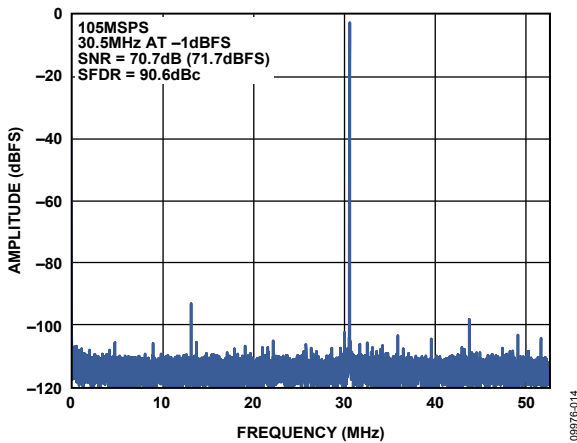
Figure 24. Single-Tone FFT with f_{IN} = 30.5 MHz
