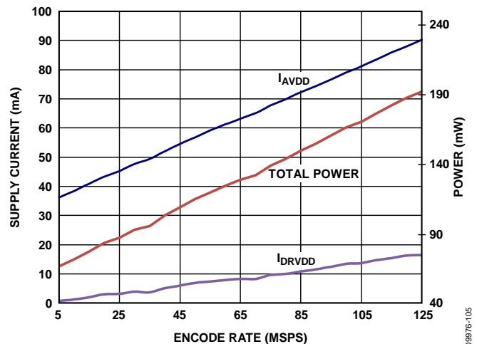
Figure 59. AD9628-125 Power and Current vs. Clock Rate (1.8 V CMOS Output Mode)
