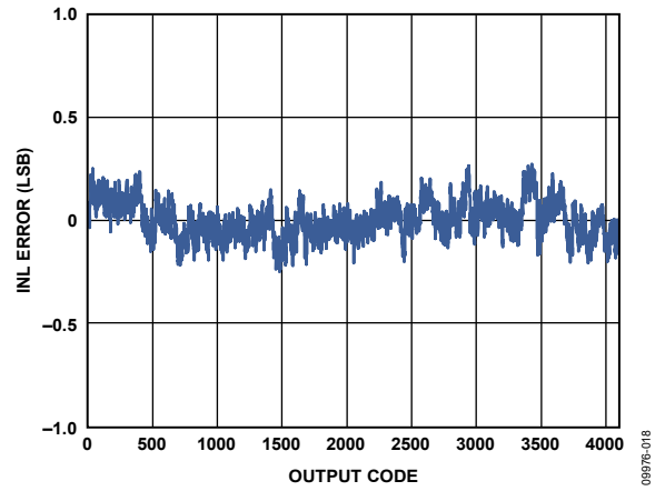
Figure 22. INL Error with f_{IN} = 9.7 MHz
