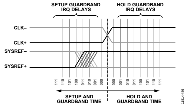
Figure 101. \text{SYSREF} \pm Edge Changes Phase Relative to the Encode Clock, Which can be Detected When the Edge Crosses Through the Guardband Setup Time
