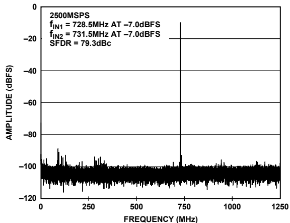
Figure 42. Two Tone FFT Plot at 2.5 GSPS, f_{IN1} = 728.5 MHz and f_{IN2} = 731.5 MHz at AIN, -7.0 dBFS (SFDR = 79.3 dBc)
