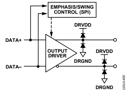
Figure 67. Digital Outputs
