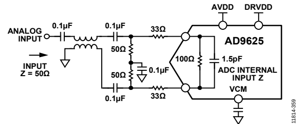
Figure 74. Input Network Example for Passive Balun with High Bandwidth
