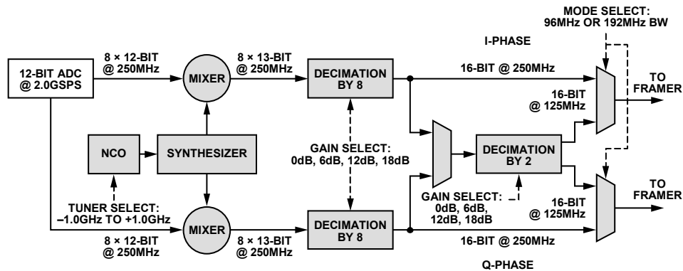
Figure 82. Digital Downconverter Block Diagram Operating at 2.0 GS/S
