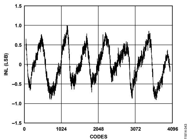
Figure 44. Integral Nonlinearity (INL), \pm 1.0 LSB at 2.5 GSps
