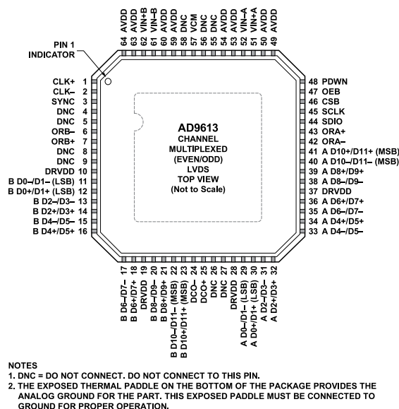
Figure 5. Pin Configuration (Top View) for the LFCSP Channel Multiplexed (Even/Odd) LVDS Mode
