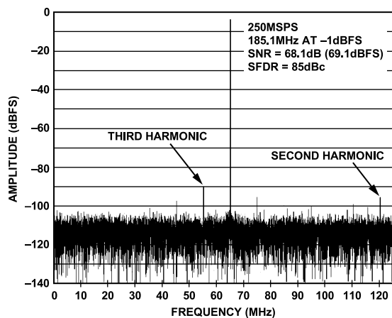
Figure 29. AD9613-250 Single-Tone FFT with f_{IN} = 185.1 MHz
