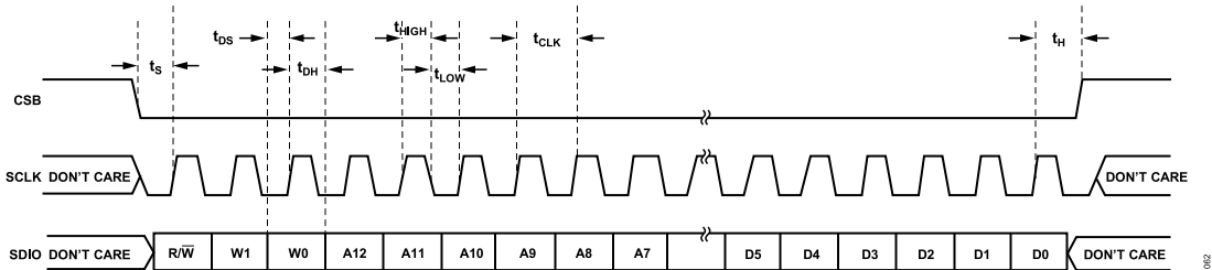
Figure 58. Serial Port Interface Timing Diagram
