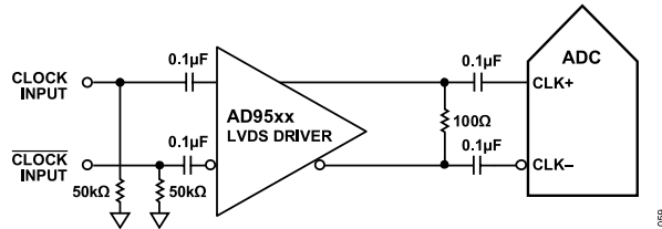
Figure 55. Differential LVDS Sample Clock (Up to 625 MHz)
