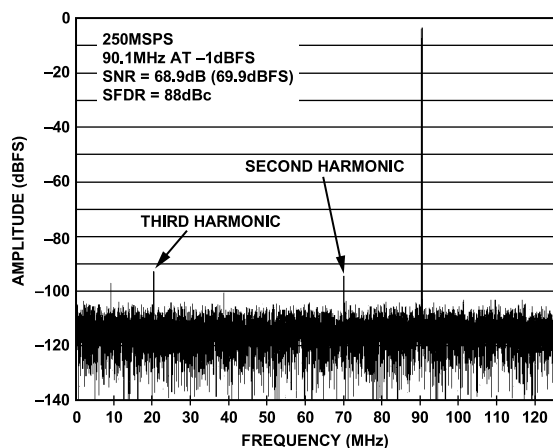
Figure 28. AD9613-250 Single-Tone FFT with f_{IN} = 90.1 MHz
