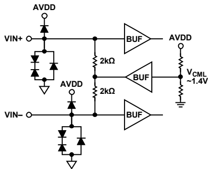
Figure 6. Analog Inputs ( V_{CML} \approx 1.4\text{ V} )
