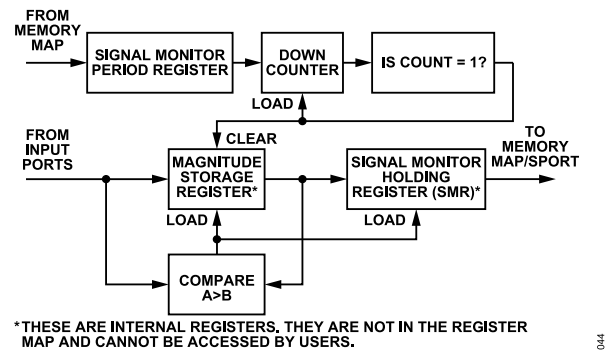
Figure 67. ADC Input Peak Detector Block Diagram
