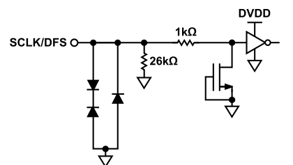
Figure 12. Equivalent SCLK/DFS Input Circuit
