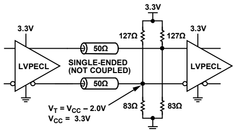
Figure 22. LVPECL Far-End Termination
