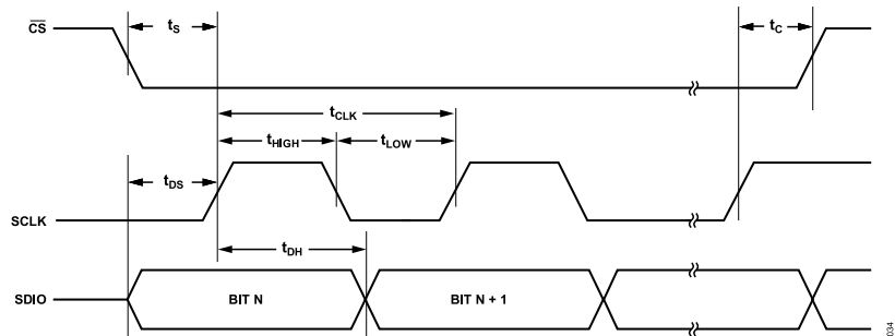
Figure 54. Serial Control Port Timing—Write
