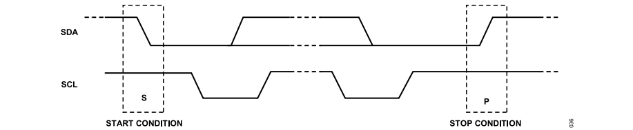
Figure 56. Start and Stop Conditions
