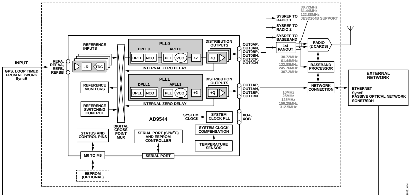
Figure 42. Small Cell Application
