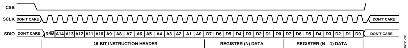
Figure 53. Serial Control Port Write—MSB First, Address Decrement, Two Bytes of Data
