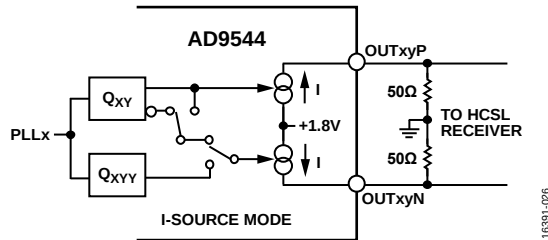
Figure 32. HCSL Output, V_{p-p} \approx 750 mV per Section ( I = 15 mA)
