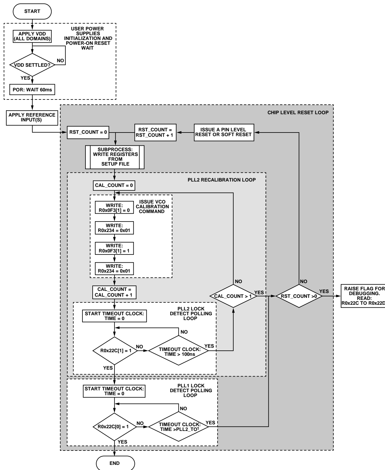
Figure 44. AD9523 Device Initialization
