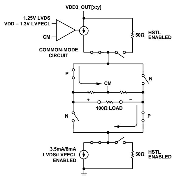
Figure 26. Multimode Driver
