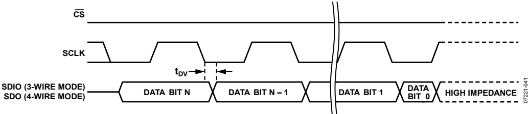
Figure 68. Timing Diagram for Serial Control Port Register Read
