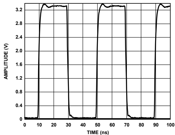
Figure 15. CMOS Output with 10 pF Load at 25 MHz
