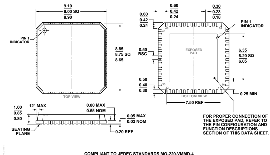
Figure 76. 64-Lead Lead Frame Chip Scale Package [LFCSP_VQ] 9 mm x 9 mm Body, Very Thin Quad CP-64-4 Dimensions shown in millimeters
