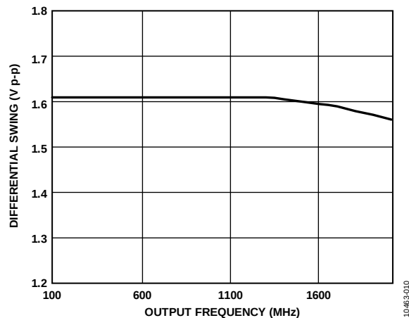
Figure 10. LVPECL Differential Output Swing vs. Frequency
