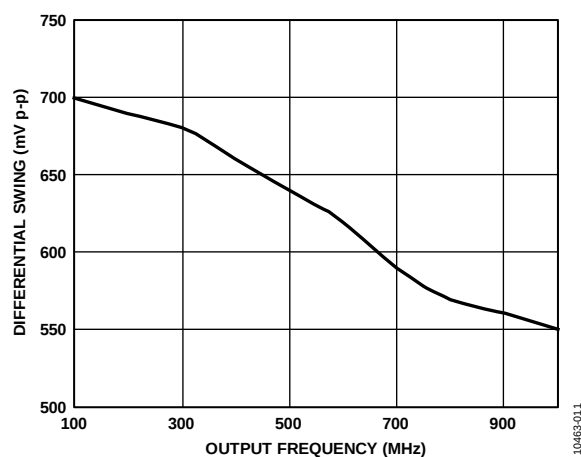
Figure 11. LVDS Differential Output Swing vs. Frequency
