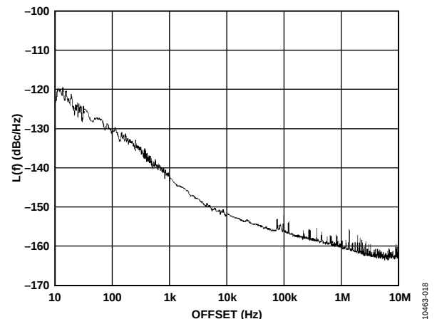
Figure 18. Additive Phase Noise—CMOS DIV4, 61.44 MHz
