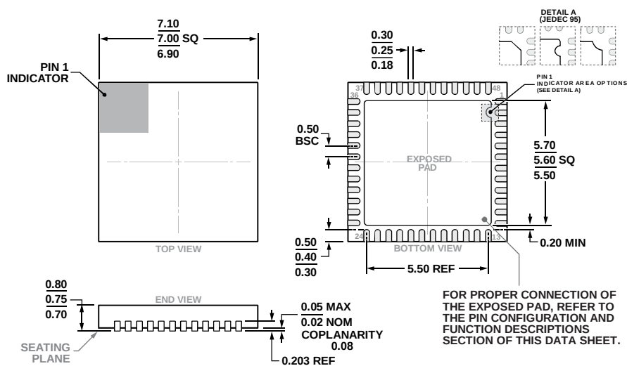
Figure 19. 48-Lead Lead Frame Chip Scale Package [LFCSP] 7 mm × 7 mm Body and 0.75 mm Package Height (CP-48-13)
