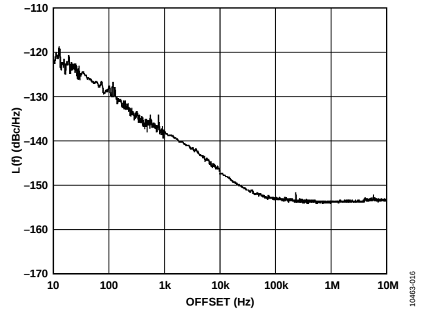
Figure 16. Additive Phase Noise—LVPECL DIV1, 622.08 MHz
