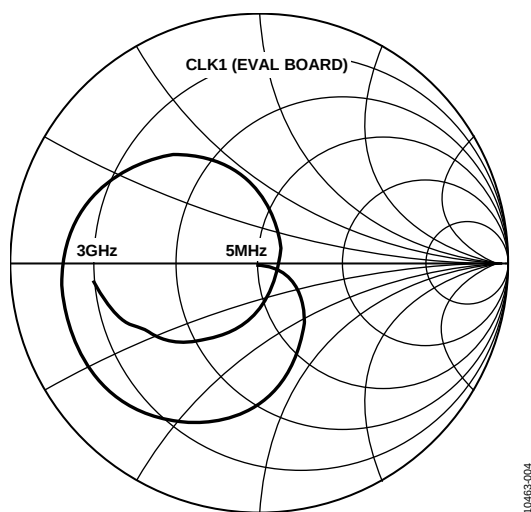
Figure 4. CLK1 Smith Chart (Evaluation Board)
