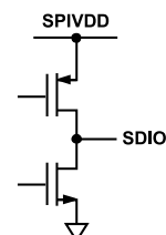
Figure 8. Equivalent SDIO Output Circuit
