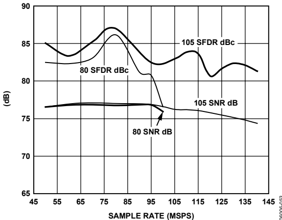
Figure 43. Single-Tone SNR/SFDR vs. Sample Rate, 170.3 MHz
