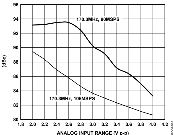
Figure 42. SFDR vs. Analog Input Range
