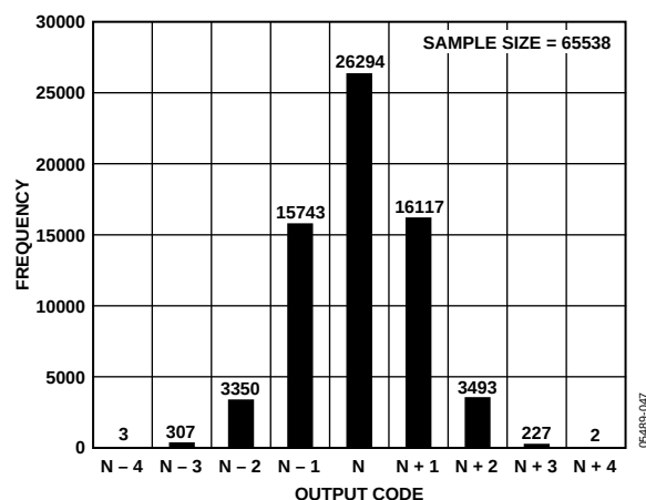
Figure 45. AD9445-105 Grounded Input Histogram
