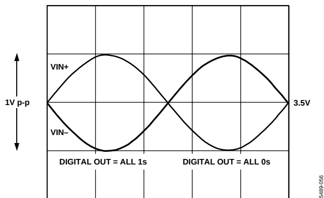
Figure 61. Differential Analog Input Range for VREF = 1.0 V
