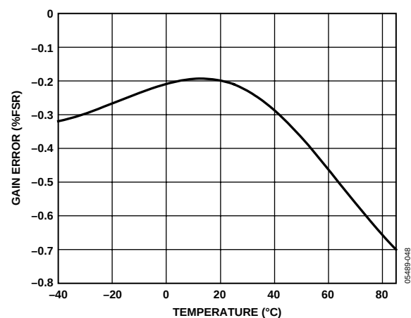
Figure 46. AD9445-125 Gain vs. Temperature
