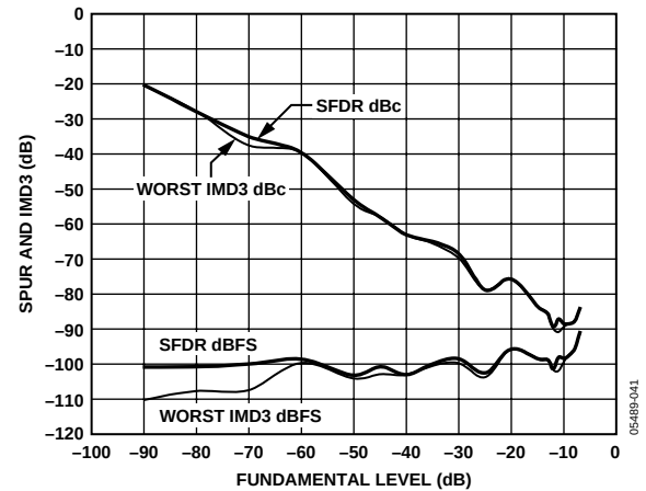
Figure 39. AD9445-125 Two-Tone SFDR vs. Analog Input Level 125 MSPS/170.3 MHz, 171.3 MHz
