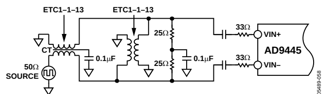
Figure 63. Double Balun-Coupled Analog Input Circuit
