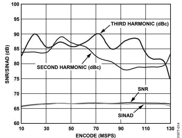
Figure 9. SNR/SINAD and Harmonic Distortion vs. Encode Frequency, Differential AIN @ -0.5 dBFS
