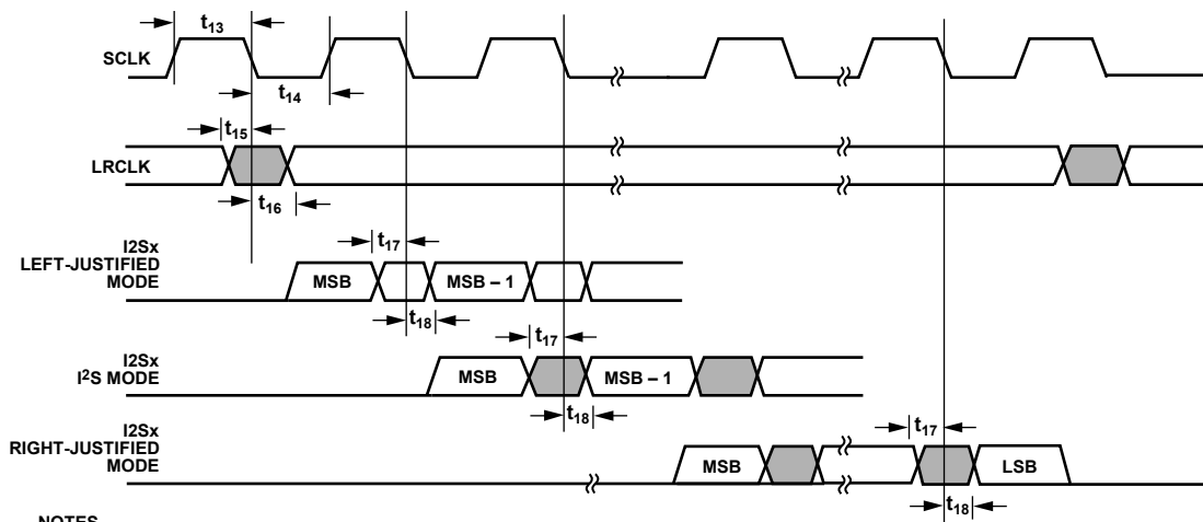
Figure 4. I²S Timing
