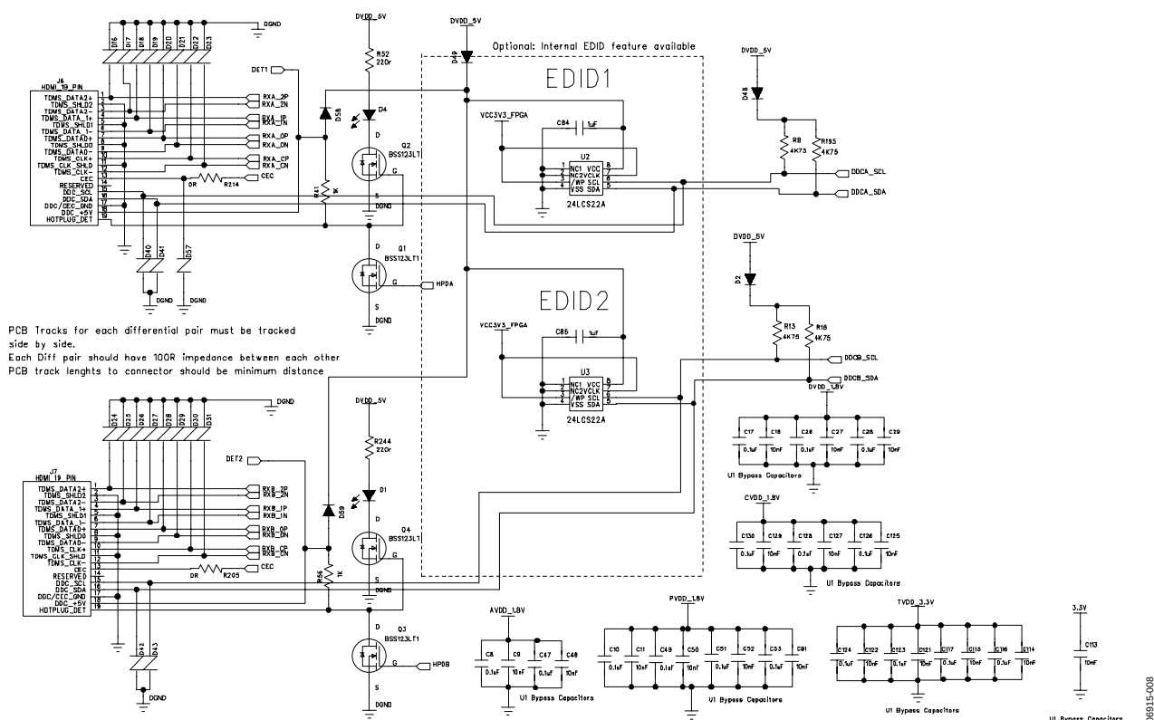
Figure 8. Typical Connection Diagram
