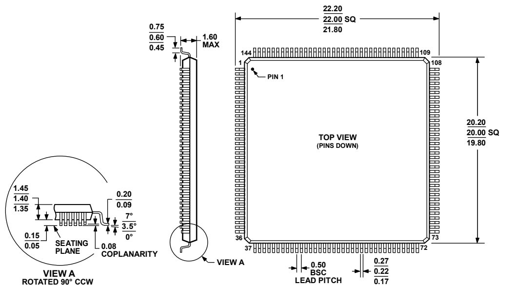
COMPLIANT TO JEDEC STANDARDS MS-026-BFB Figure 12. 144-Lead Low Profile Quad Flat Package [LQFP] (ST-144) Dimensions shown in millimeters
