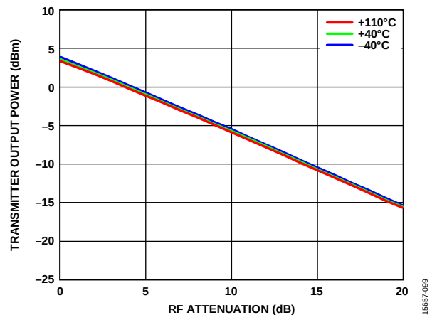
Figure 158. Transmitter Output Power vs. RF Attenuation, 3500 MHz LO, 3505 MHz CW Desired Signal, 100 MHz RF Bandwidth, 2 dB Digital Backoff, 307.2 MSPS Sample Rate
