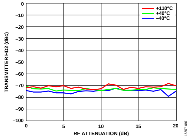
Figure 156. Transmitter HD2 vs. RF Attenuation, 3500 MHz LO, 3505 MHz CW Desired Signal, 100 MHz RF Bandwidth, 307.2 MSPS Sample Rate
