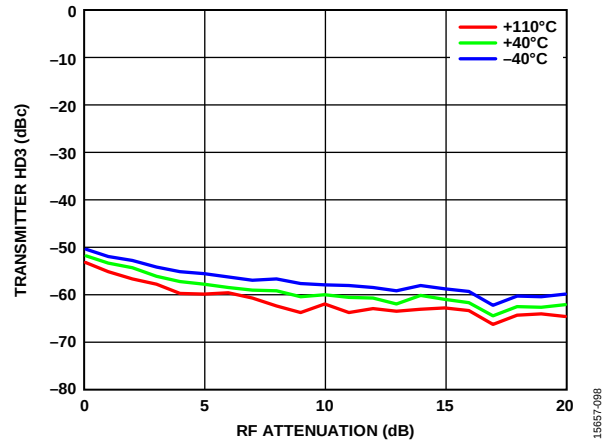
Figure 157. Transmitter HD3 vs. RF Attenuation, 3500 MHz LO, 3505 MHz CW Desired Signal, 100 MHz RF Bandwidth, 307.2 MSPS Sample Rate
