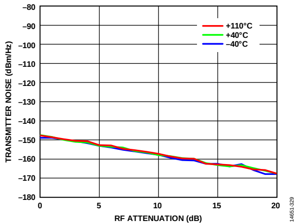
Figure 29. Transmitter Noise vs. RF Attenuation, 800 MHz LO, 20 MHz Offset Frequency
