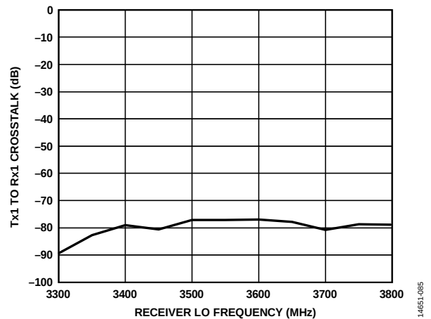
Figure 144. Tx1 to Rx1 Crosstalk vs. Receiver LO Frequency, 100 MHz Receiver RF Bandwidth, 100 MHz Transmitter RF Bandwidth, CW Signal 3 MHz Offset from LO
