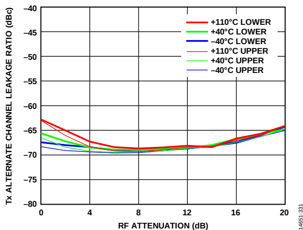
Figure 31. Tx Alternate Channel Leakage Ratio vs. RF Attenuation, 900 MHz LO, 20 MHz RF Bandwidth, Four-Carrier W-CDMA Desired Signal, 2 dB Digital Backoff, Transmitter QEC and LO Leakage Tracking Active
