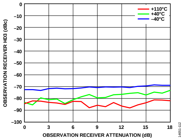
Figure 171. Observation Receiver HD3 vs. Observation Receiver Attenuation, 3500 MHz LO, CW Signal 25 MHz Offset, -20 dBm at 0 dB Attenuation, Input Power Increasing Decibel for Decibel with Attenuation, 240 MHz RF Bandwidth, 307.2 MSPS Sample Rate
