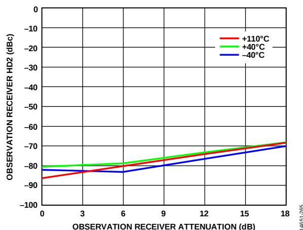
Figure 228. Observation Receiver HD2 vs. Observation Receiver Attenuation, 5600 MHz LO, CW Signal 30 MHz Offset, -15 dBm Input, Input Power Increasing Decibel for Decibel with Attenuation, 200 MHz RF Bandwidth, 245.76 MSPS Sample Rate
