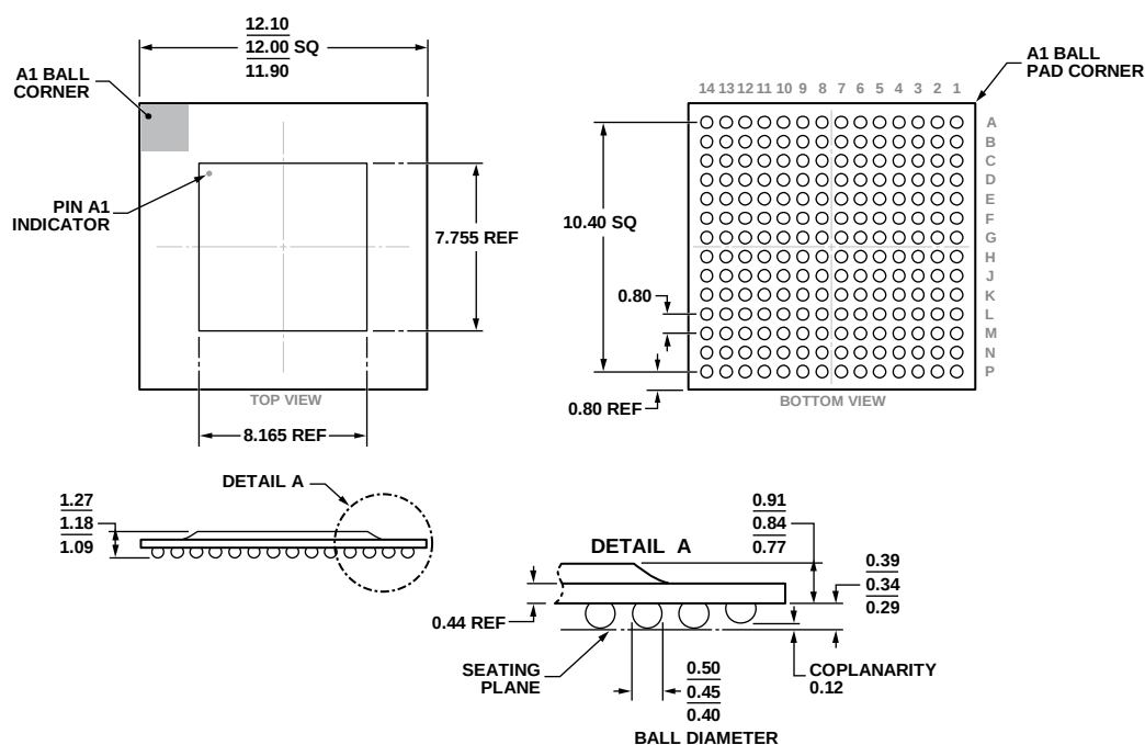
Figure 232. 196-Ball Chip Scale Package Ball Grid Array [CSP_BGA] (BC-196-12)
