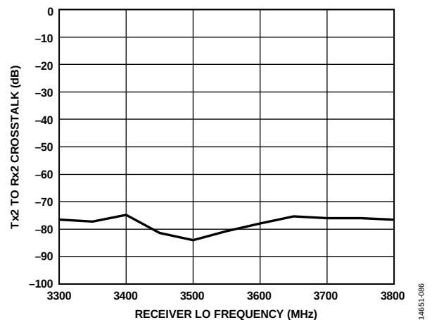
Figure 145. Tx2 to Rx2 Crosstalk vs. Receiver LO Frequency, 100 MHz Receiver RF Bandwidth, 100 MHz Transmitter RF Bandwidth, CW Signal 3 MHz Offset from LO
