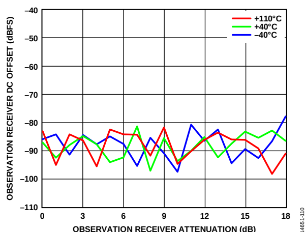
Figure 169. Observation Receiver DC Offset vs. Observation Receiver Attenuation, 3500 MHz LO, 240 MHz RF Bandwidth, 307.2 MSPS Sample Rate
