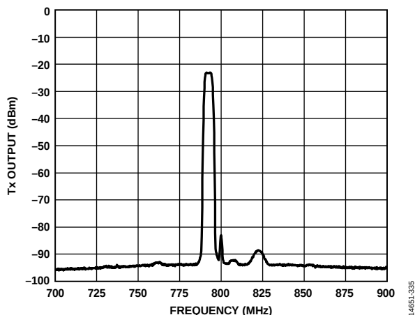
Figure 35. Tx Output Power Spectrum, 2 dB Digital and 3 dB RF Backoff, 20 MHz RF Bandwidth, Transmitter QEC, and Internal LO Leakage Active, LTE 10 MHz Signal, 800 MHz LO, 1 MHz Resolution Bandwidth, 122.88 MSPS Sample Rate, Test Equipment Noise Floor De-Embedded
