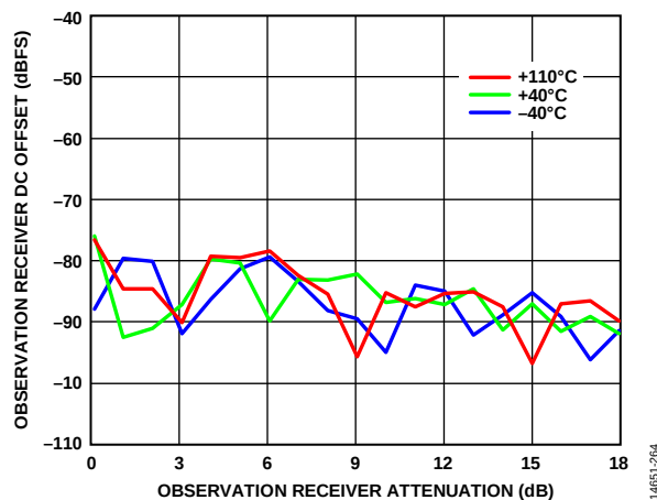
Figure 227. Observation Receiver DC Offset vs. Observation Receiver Attenuation, 5850 MHz LO, CW Signal 30 MHz Offset, -15 dBm Input, 200 MHz RF Bandwidth, 245.76 MSPS Sample Rate
