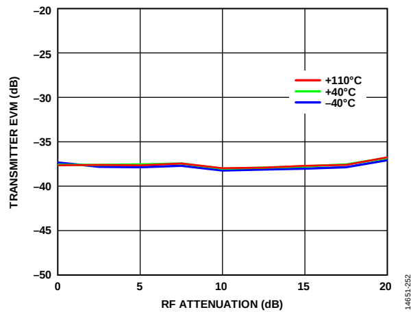
Figure 213. Transmitter EVM vs. RF Attenuation, 5600 MHz LO, Transmitter LO Leakage, and Transmitter QEC Tracking Active, 75 MHz RF Bandwidth, LTE 20 MHz Downlink Signal, 245.76 MSPS Sample Rate
