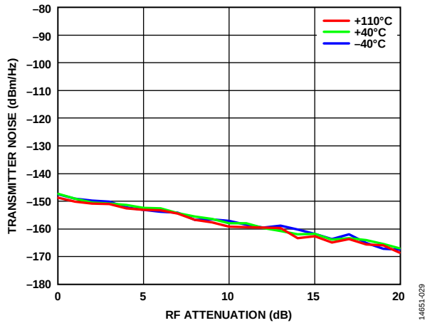
Figure 88. Transmitter Noise vs. RF Attenuation, 2600 MHz LO, 10 MHz Offset Frequency
