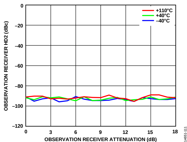
Figure 170. Observation Receiver HD2 vs. Observation Receiver Attenuation, 3500 MHz LO, CW Signal 25 MHz Offset, -20 dBm at 0 dB Attenuation, Input Power Increasing Decibel for Decibel with Attenuation, 240 MHz RF Bandwidth, 307.2 MSPS Sample Rate
