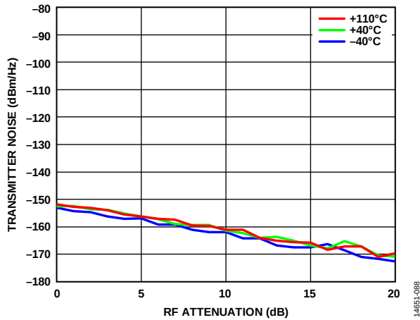
Figure 147. Transmitter Noise vs. RF Attenuation, 3500 MHz LO, 100 MHz Offset Frequency, Zeros Input Data
