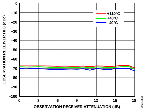
Figure 53. Observation Receiver HD3 vs. Observation Receiver Attenuation, 800 MHz LO, CW Signal 16 MHz Offset, -20 dBm at 0 dB Attenuation, Input Power Increasing Decibel for Decibel with Attenuation, 100 MHz RF Bandwidth, 122.88 MSPS Sample Rate
