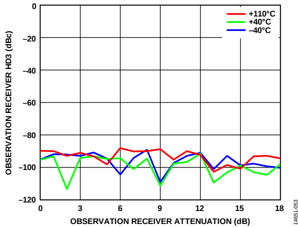
Figure 112. Observation Receiver HD3 vs. Observation Receiver Attenuation, 2600 MHz LO, CW Signal 25 MHz Offset, -20 dBm at 0 dB Attenuation, Input Power Increasing Decibel for Decibel with Attenuation, 200 MHz RF Bandwidth, 245.76 MSPS Sample Rate
