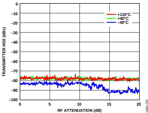
Figure 214. Transmitter HD2 vs. RF Attenuation, 5850 MHz LO, 5855 MHz CW Desired Signal, 75 MHz RF Bandwidth, 245.76 MSPS Sample Rate
