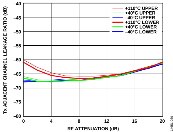
Figure 89. Tx Adjacent Channel Leakage Ratio vs. RF Attenuation, 2600 MHz LO, 40 MHz RF Bandwidth, Four-Carrier W-CDMA Desired Signal, Transmitter QEC and LO Leakage Tracking Active
