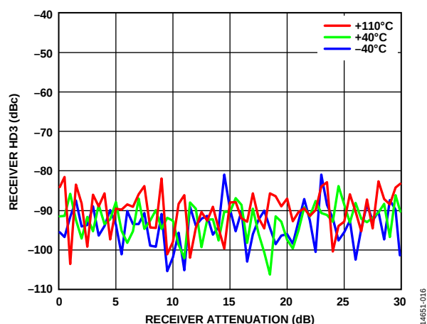
Figure 75. Receiver HD3 vs. Receiver Attenuation, 2600 MHz LO, CW Signal 5 MHz Offset, -20 dBm at 0 dB Attenuation, Input Power Increasing Decibel for Decibel with Attenuation, 40 MHz RF Bandwidth, 122.88 MSPS Sample Rate
