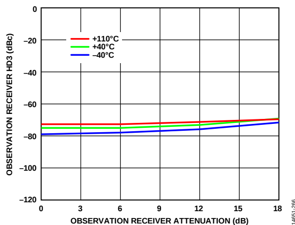
Figure 229. Observation Receiver HD3 vs. Observation Receiver Attenuation, 5600 MHz LO, CW Signal 30 MHz Offset, -15 dBm Input, Input Power Increasing Decibel for Decibel with Attenuation, 200 MHz RF Bandwidth, 245.76 MSPS Sample Rate
