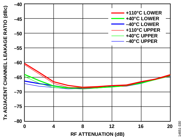
Figure 30. Tx Adjacent Channel Leakage Ratio vs. RF Attenuation, 900 MHz LO, 20 MHz RF Bandwidth, Four-Carrier W-CDMA Desired Signal, Transmitter QEC and LO Leakage Tracking Active
