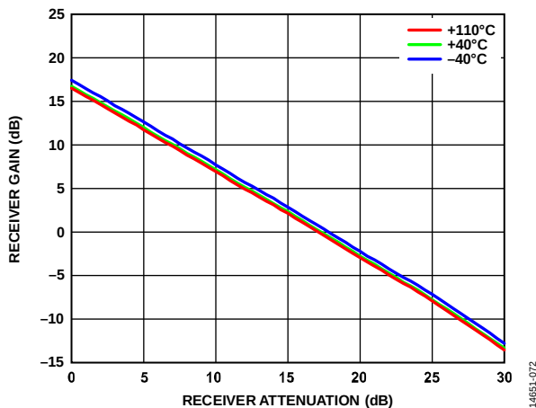
Figure 131. Receiver Gain vs. Receiver Attenuation, 3500 MHz LO, CW Signal 17 MHz Offset, 100 MHz RF Bandwidth, De-Embedded to Receiver Port, 153.6 MSPS Sample Rate
