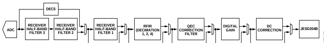
Figure 231. Data Rx Data Path Filter Implementation
