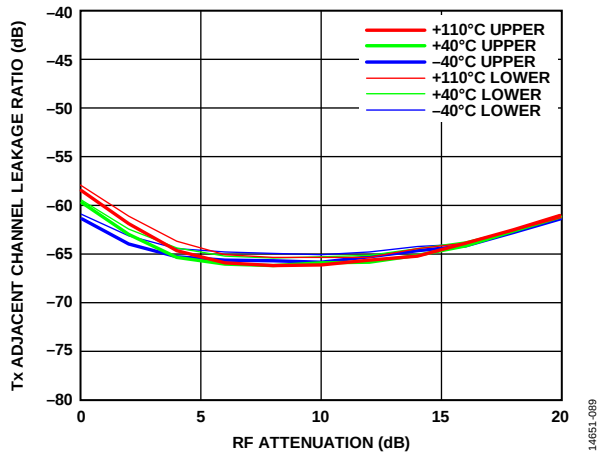
Figure 148. Tx Adjacent Channel Leakage Ratio vs. RF Attenuation, 3500 MHz LO, 100 MHz RF Bandwidth, Four-Carrier W-CDMA Desired Signal, 2 dB Digital Backoff, Transmitter QEC and LO Leakage Tracking Active
