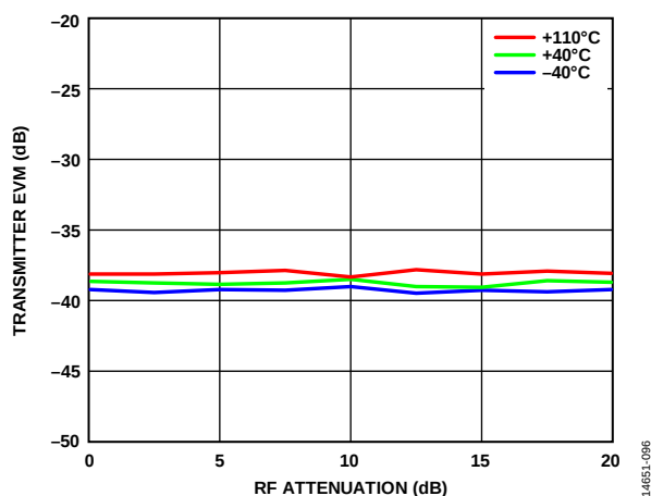
Figure 155. Transmitter EVM vs. RF Attenuation, 3500 MHz LO, Transmitter LO Leakage, and Transmitter QEC Tracking Active, 100 MHz RF Bandwidth, LTE 20 MHz Downlink Signal, 307.2 MSPS Sample Rate
