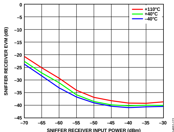
Figure 180. Sniffer Receiver EVM vs. Sniffer Receiver Input Power, 3600 MHz LO, 20 MHz RF Bandwidth, LTE 20 MHz Uplink Centered at DC, BTC Active, 38.4 MSPS Sample Rate
