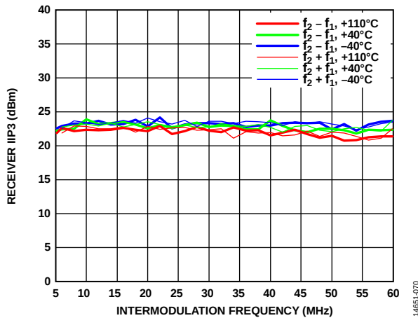
Figure 129. Receiver IIP3 vs. Intermodulation Frequency, 3500 MHz LO, 0 dB Attenuation, 100 MHz RF Bandwidth, 153.6 MSPS Sample Rate
