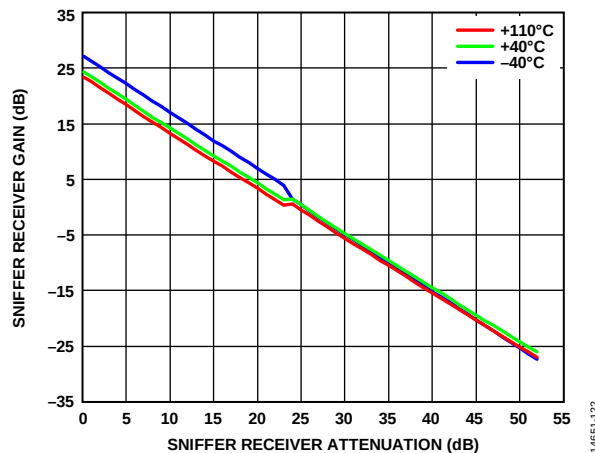
Figure 181. Sniffer Receiver Gain vs. Sniffer Receiver Attenuation, 3600 MHz LO, CW Signal 5 MHz Offset, 20 MHz RF Bandwidth, De-Embedded to Receiver Port, 38.4 MSPS Sample Rate
