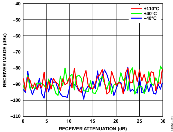
Figure 130. Receiver Image vs. Receiver Attenuation, 3500 MHz LO, Continuous Wave (CW) Signal 17 MHz Offset, 100 MHz RF Bandwidth, Background Tracking Calibration (BTC) Active, 153.6 MSPS Sample Rate
