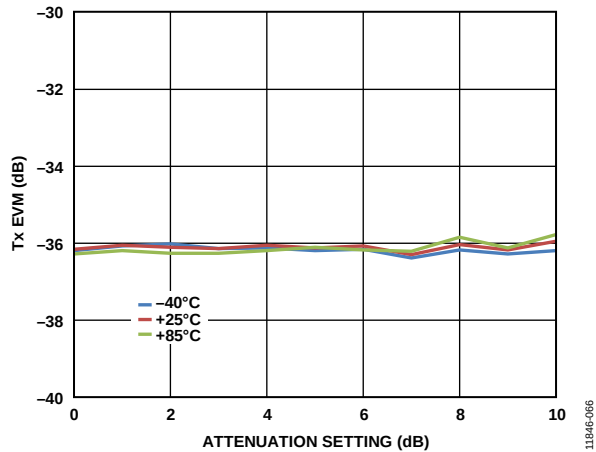
Figure 66. Tx EVM vs. Transmitter Attenuation Setting, WiMAX 40 MHz, 64 QAM Modulation, f_{LO\_TX} = 5.495 GHz, 40 MHz REF_CLK (Doubled Internally for RF Synthesizer)
