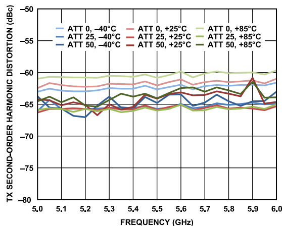
Figure 69. TX Second-Order Harmonic Distortion (HD2) vs. Frequency
