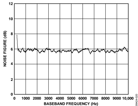
Figure 21. Noise Figure vs. Baseband Frequency
