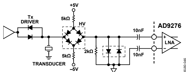
Figure 52. Input Overload Protection
