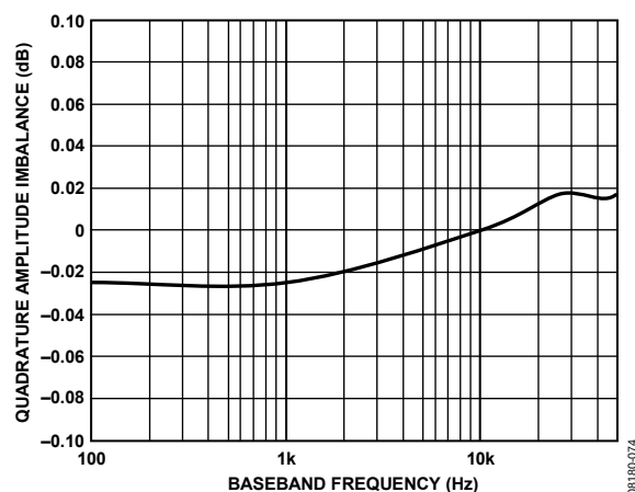
Figure 24. Quadrature Amplitude Imbalance vs. Baseband Frequency
