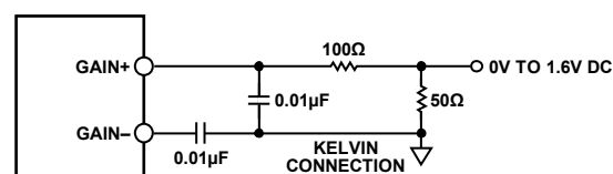
Figure 60. Single-Ended \text{GAIN}+ , \text{GAIN}- Pin Configuration
