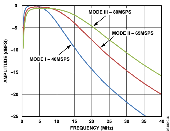
Figure 16. Antialiasing Filter (AAF) Pass-Band Response, LPF\text{ Cutoff} = f_{SAMPLE}/3 (Mode I and Mode II), f_{SAMPLE}/4.5 (Mode III)
