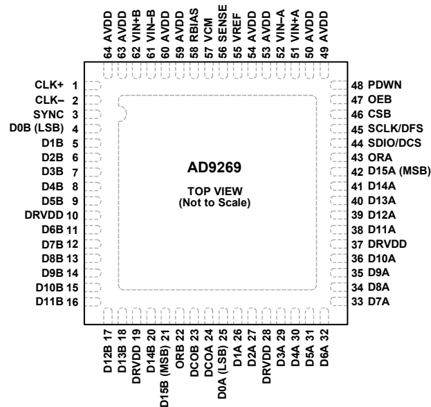
Figure 5. Pin Configuration
