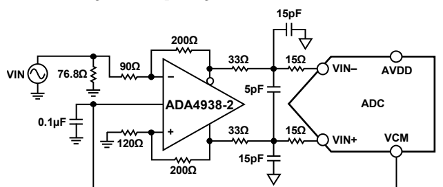
Figure 66. Differential Input Configuration Using the ADA4938-2
