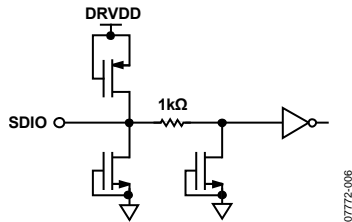
Figure 32. Equivalent SDIO Input Circuit
