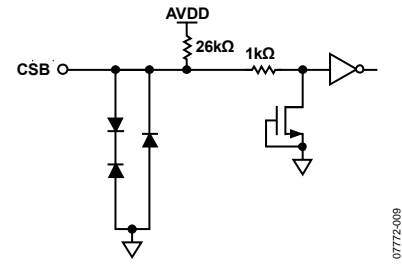
Figure 34. Equivalent CSB Input Circuit
