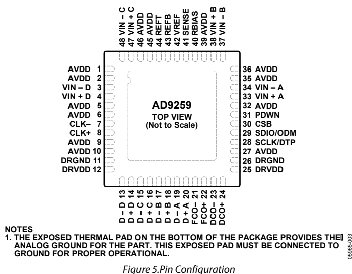
Figure 5. Pin Configuration
