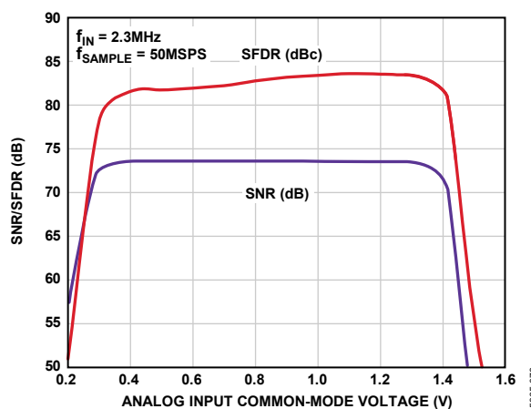
Figure 36. SNR/SFDR vs. Common-Mode Voltage, f_{IN} = 2.3 \text{ MHz} , f_{SAMPLE} = 50 \text{ MSPS}
