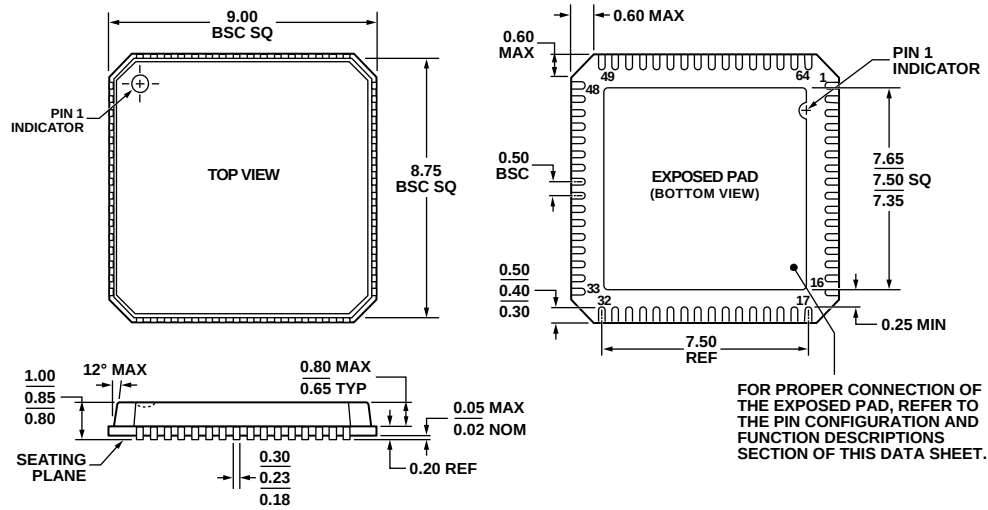
Figure 85. 64-Lead Lead Frame Chip Scale Package [LFCSP_VQ] 9 mm x 9 mm Body, Very Thin Quad (CP-64-6) Dimensions shown in millimeters
