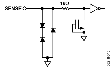
Figure 10. Equivalent Sense Circuit
