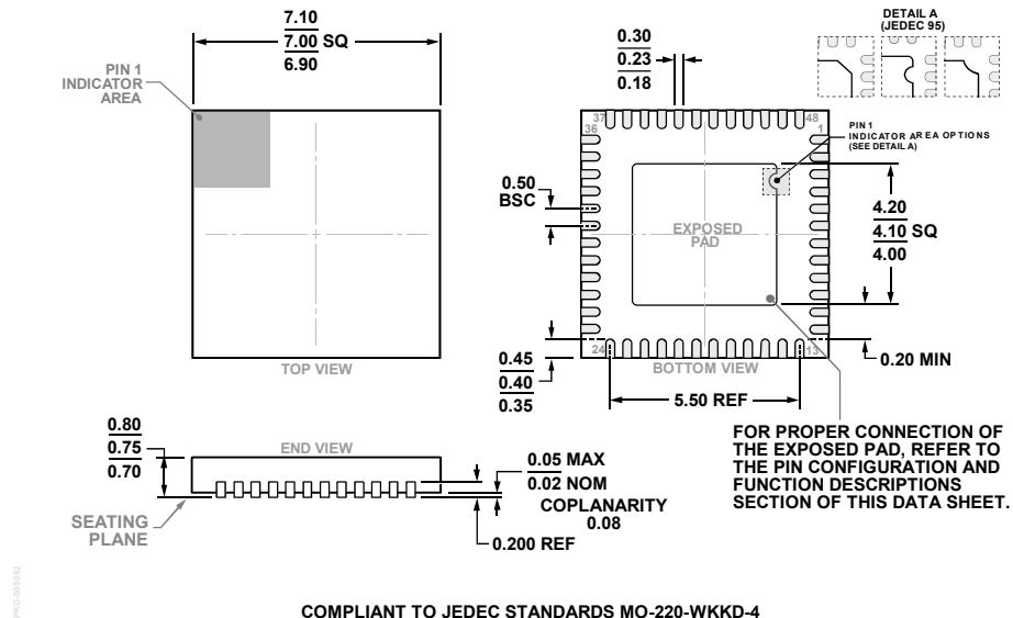
Figure 64. 48-Lead Lead Frame Chip Scale Package [LFCSP] 7 mm × 7 mm Body and 0.75 mm Package Height (CP-48-5)
