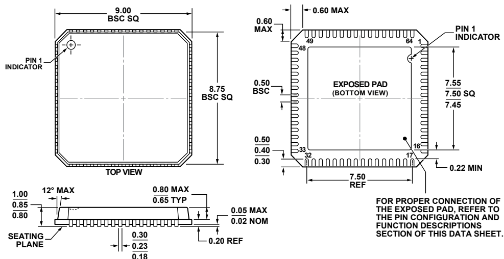
Figure 73. 64-Lead Lead Frame Chip Scale Package [LFCSP_VQ]
