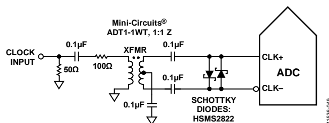
Figure 39. Transformer-Coupled Differential Clock (Up to 200 MHz)
