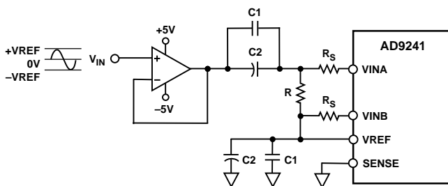
Figure 34. AC-Coupled Input
