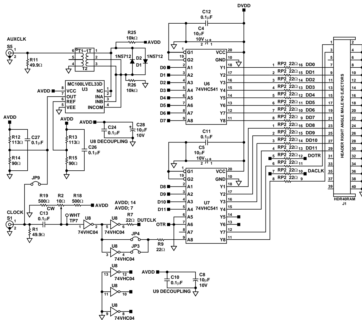
Figure 45. TSSOP Evaluation Board Schematic, Clock Inputs and Output Buffering
