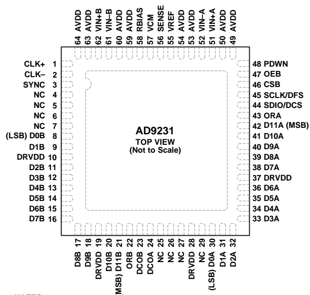
Figure 5. Pin Configuration
